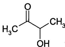
Acetoin (acetyl methyl carbinol) C_4H_8O_2
