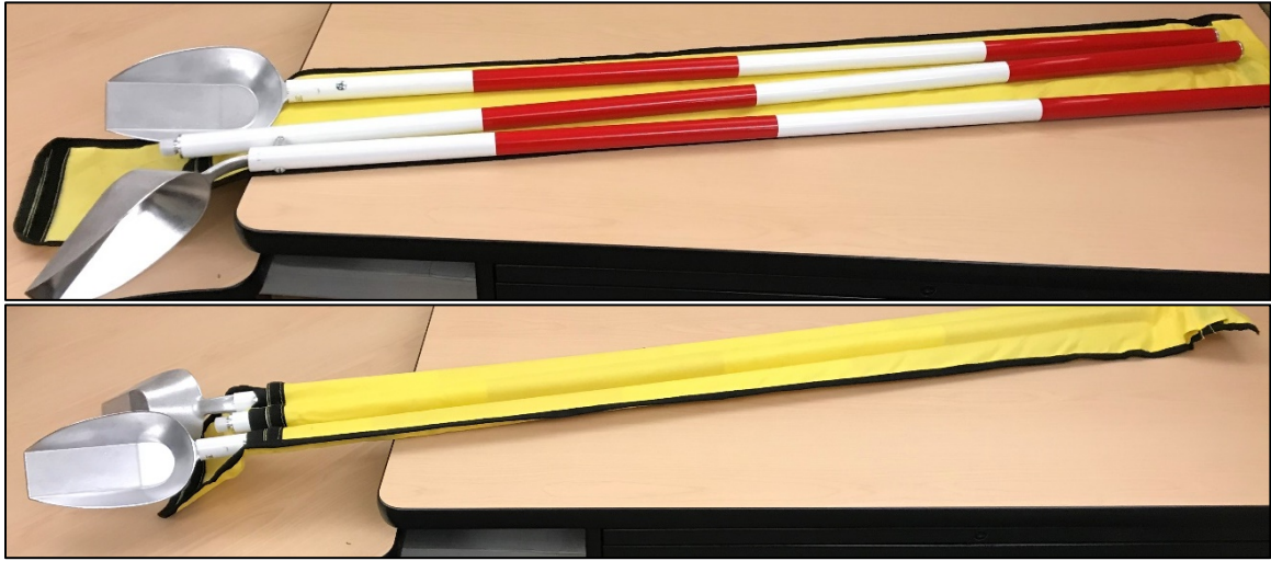
Figure VIII-7: Non-sparking, aluminum extension scoop assembly. (Source: OSHA HRT)
