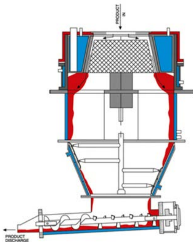
Gap Mill (Source: http://www.chocolatemixer.in/gapmill.html )
